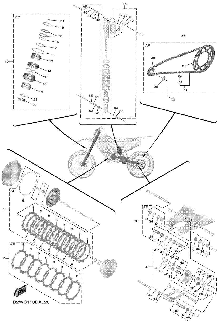
FIG. 2 MAINTENANCE PARTS KIT
