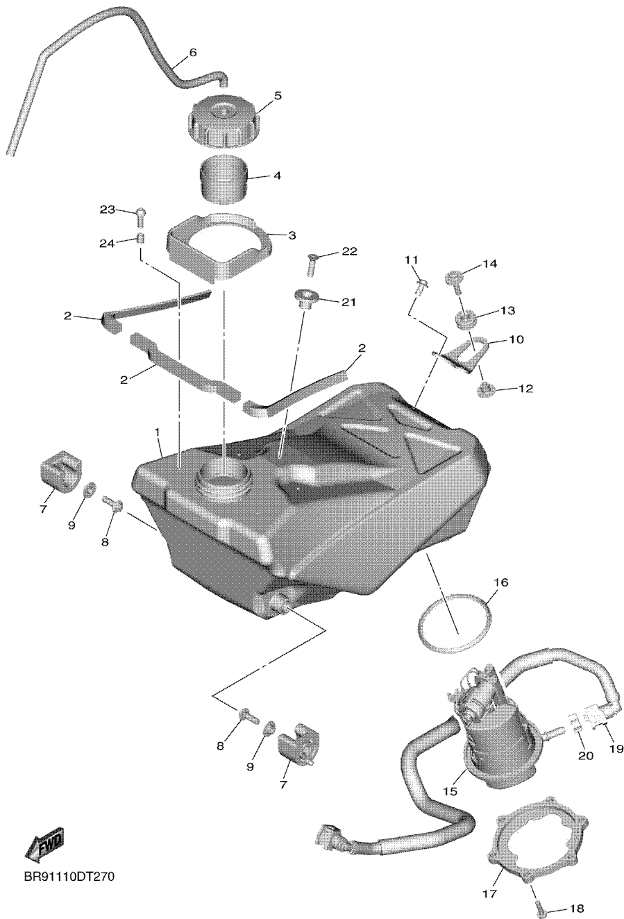
FIG. 30 FUEL TANK
